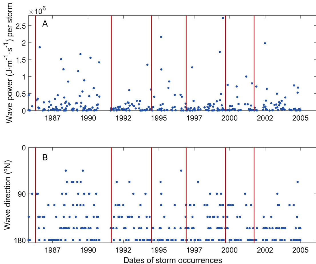
Fig. 8. Storm waves between 1985 and 2005 from the Sydney wave rider buoy showing A) Total wave power and B) Wave direction. Storm waves do not occur beyond 180^{\circ} due to shoreline orientation. Red vertical lines correspond to dates of aerial photos used in this study. (For interpretation of the references to colour in this figure legend, the reader is referred to the Web version of this article.)
