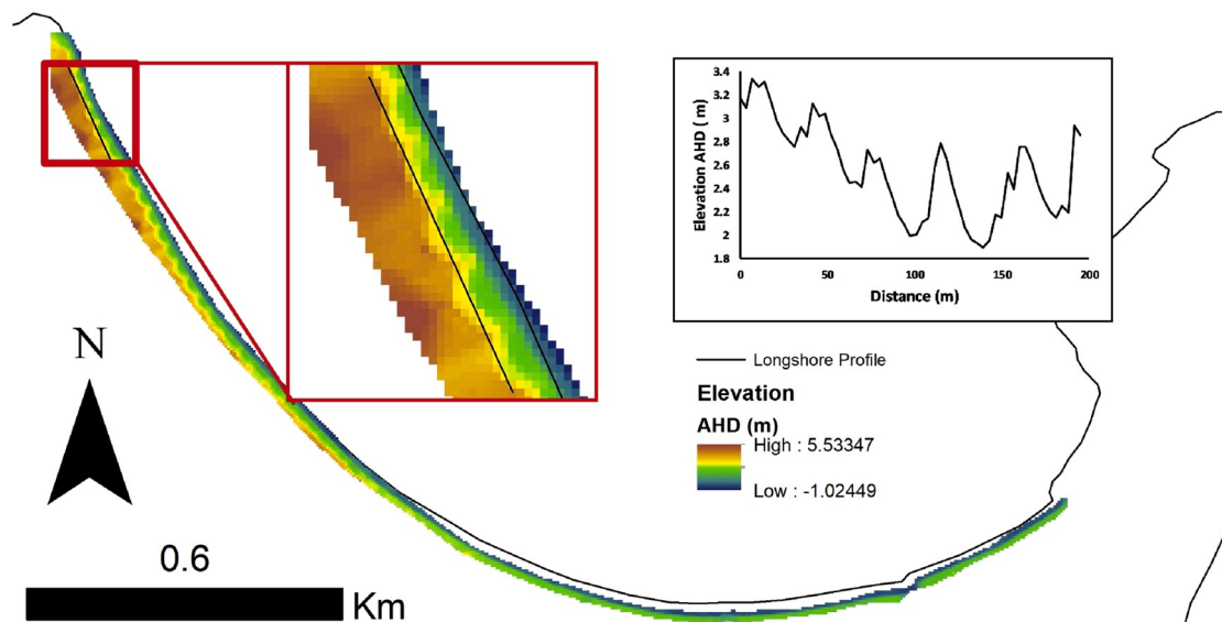
Fig. 6. Digital elevation model (DEM) of Shoal Bay beach during May 2009 with beach cusps apparent in the western area of the beach. A longshore profile shows the beach cusps that occur on the western area of the beach.
