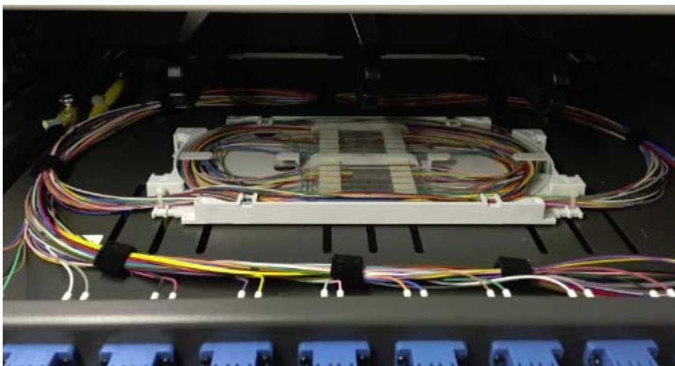
Image 2 - 48 Core Fibre Optic Breakout tray in Floor Distributor cabinet
