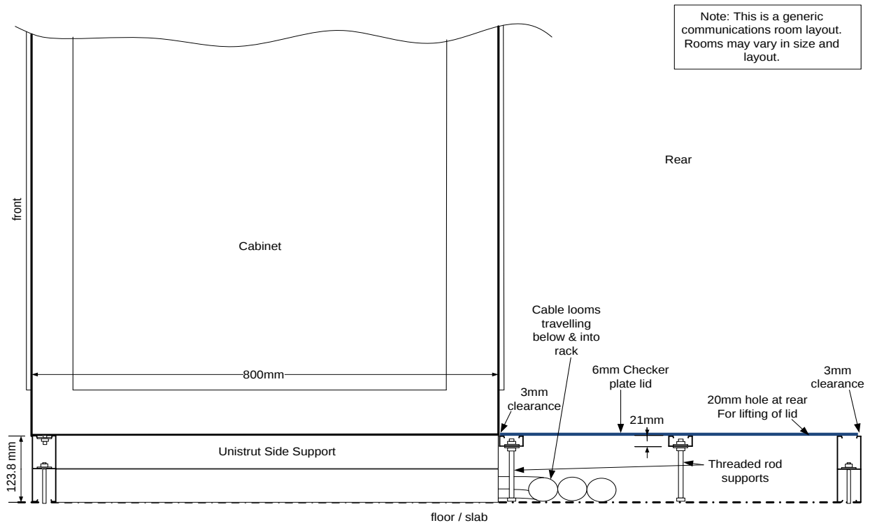
Side View Underfloor cabinet design for 123.8 mm Unistrut
